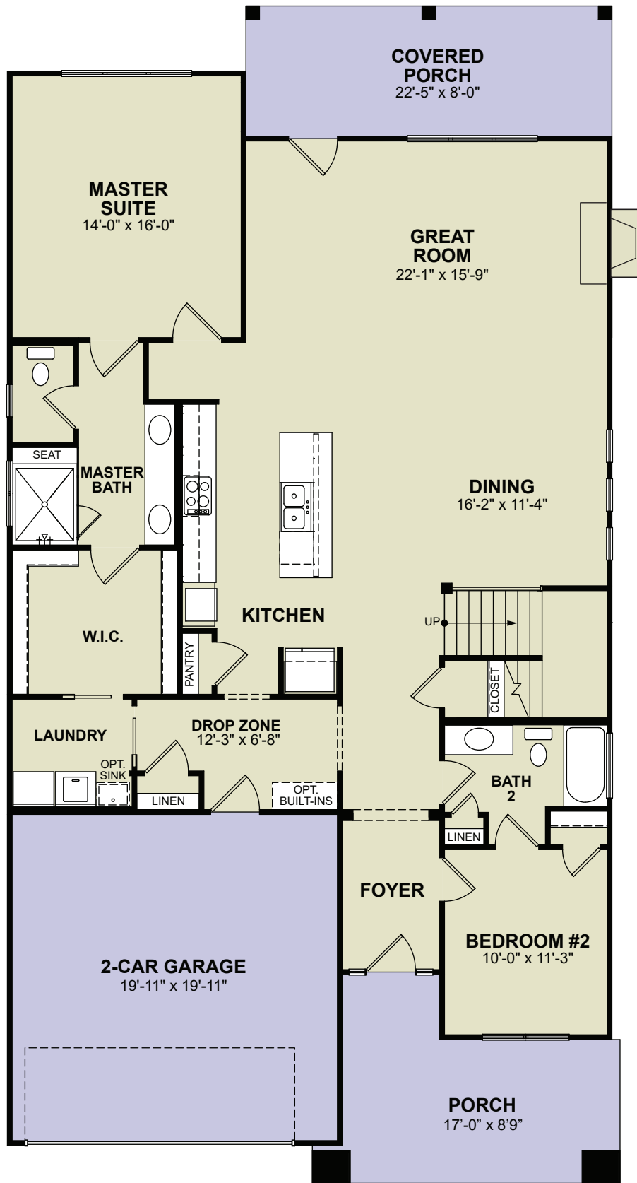
FIRST FLOOR
