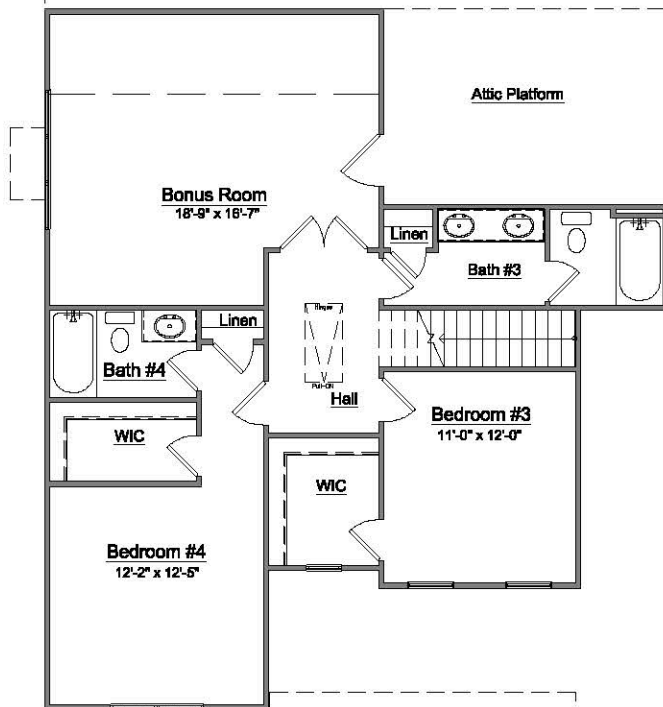
Second Floorplan
