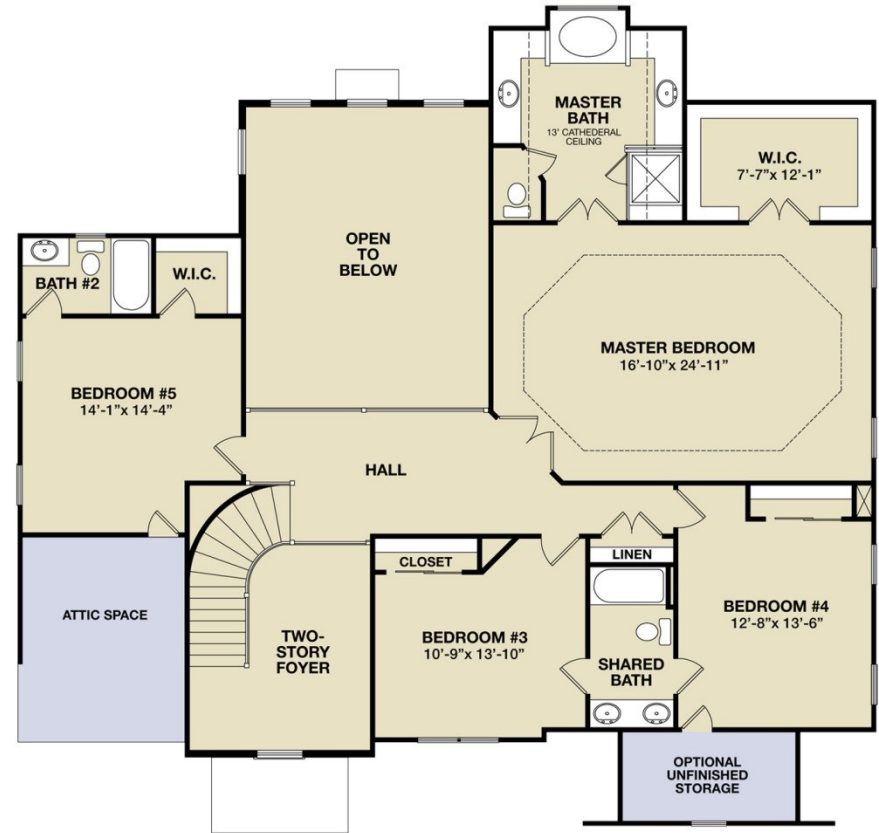
Second Floor
