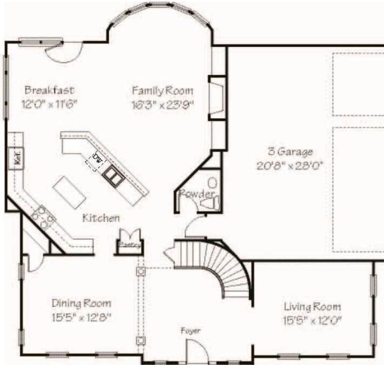
1st floor
