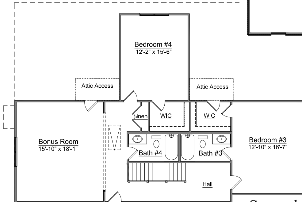
Second Floor
