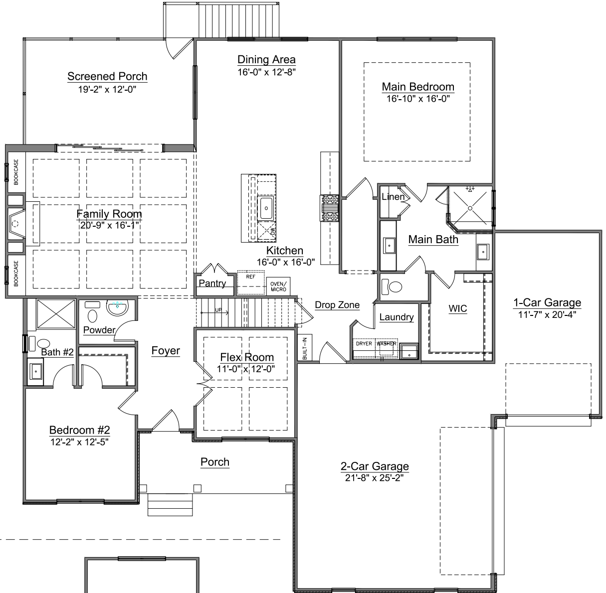
First Floor
